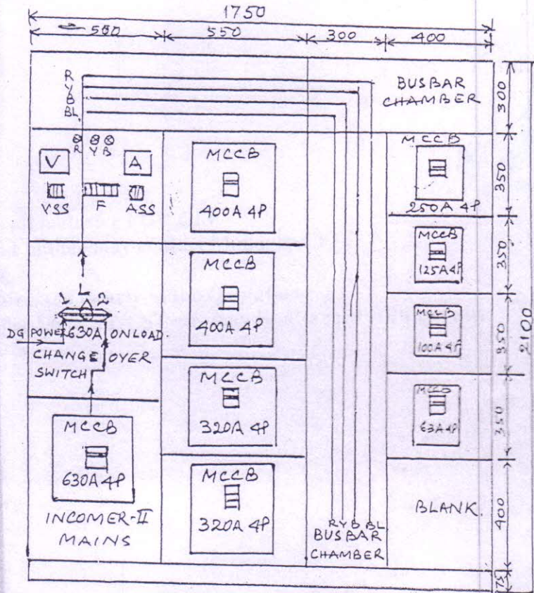
FRONT VIEW POWER DISTRIBUTION PANEL FOR OLD PLANT DIMENSION - 1750X2100X1000MM
