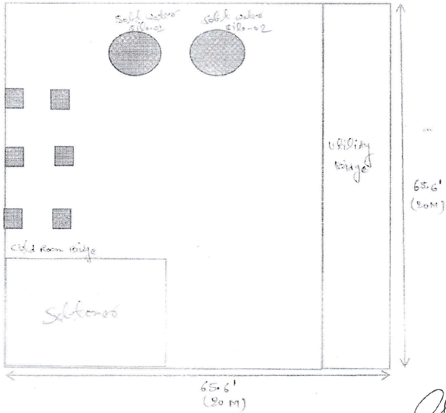
PROPOSED PLAN OF CONCRETING AREA AROUND SOFTWATER SILOS
